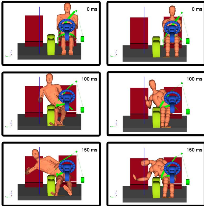
Figure 5. MADYMO Human Facet Model and Hybrid III Model Subjected to Adjusted IIHS Crash Pulse with Intrusion Predicted by FEM Model Shown as Vertical Line
