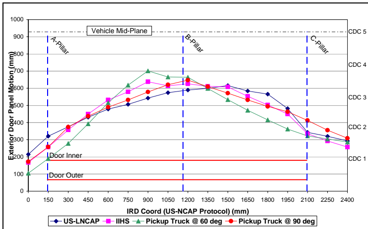
Figure 4. Comparisons of the Taurus Side Deformation (elastic plus plastic) at the Window Sill Level after Simulated Impacts by the NHTSA Barrier, the IIHS Barrier, and a C-1500 pickup
