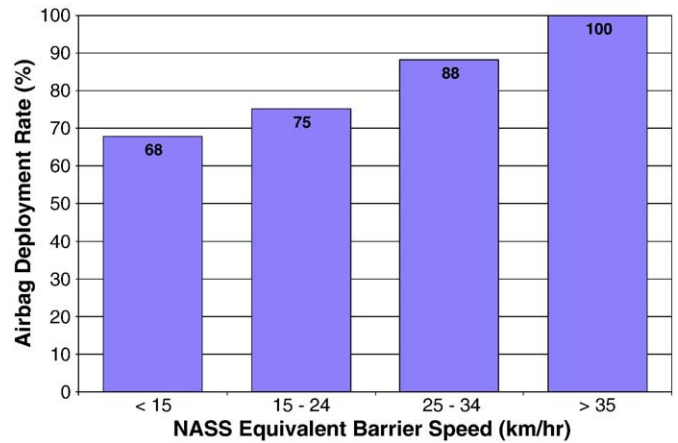
Fig. 2. Airbag Deployment as a Function of Equivalent Barrier Speed in Longitudinal Barrier Crashes involving only Airbag-Equipped Vehicles. [NASS/CDS 1997–2007, inclusive].
