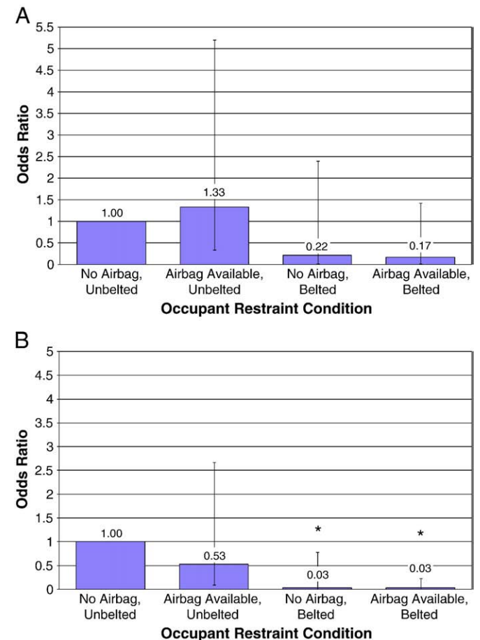
Fig. 4. Equivalent Barrier Speed Adjusted Odds Ratio and 95% Confidence Interval Plot for Longitudinal Barrier Crash Occupant Injury by Restraint Condition (n = 413): MAIS 2+ (A) and MAIS 3+ (B). [NASS/CDS 1997–2007, inclusive].
