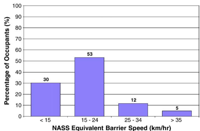
Fig. 3. Distribution of Equivalent Barrier Speeds for All Available Longitudinal Barrier Crashes. [NASS/CDS 1997–2007, inclusive].
