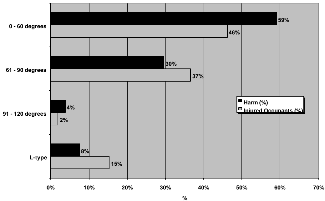
Figure 7. Distribution of pole-to-car side impacts by impact location and angle (CVF 1989-92)
