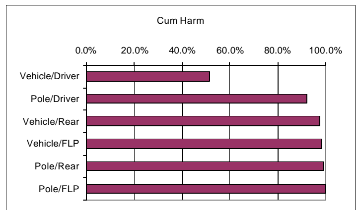
Figure 11 Cumulative Harm distribution in far-side crashes
