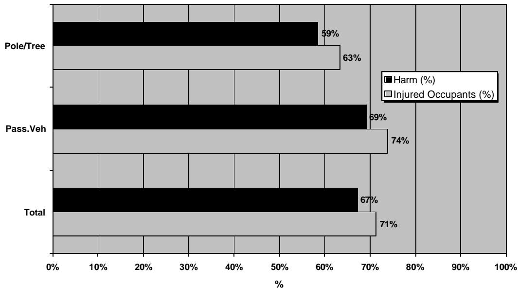
Figure 8. Near- versus Far-side Impacts (CVF 1989-92)
