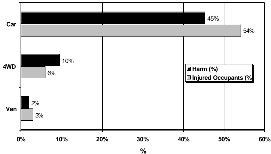
Figure 3 Distribution of Side Impacts by Striking Vehicle/Object (CVF 1989-92)
