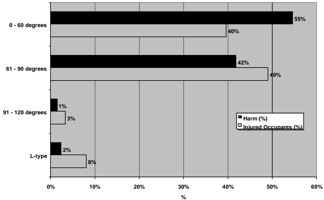
Figure 6. Distribution of vehicle-to-car side impacts by impact location and angle (CVF 1989-92)
