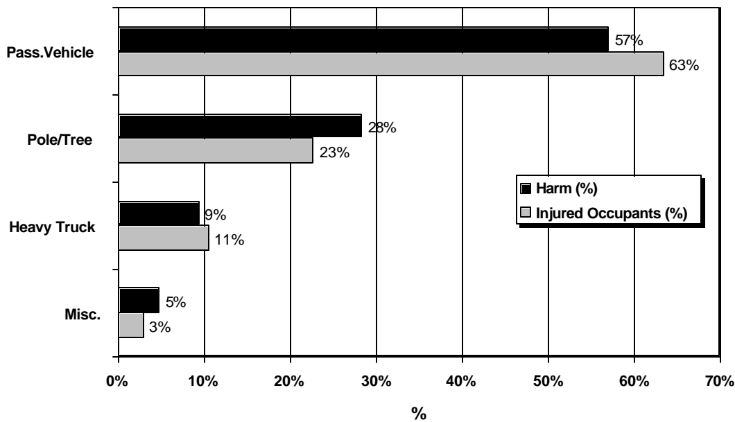
Figure 2 Distribution of Side Impacts by Striking Vehicle/Object (CVF 1989-92)
